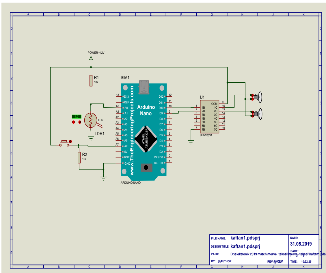
Figure 13. Electronic schematic of sensor system
